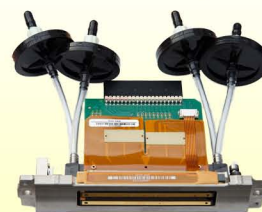
SPECTRA Polaris Print Head 35pl
